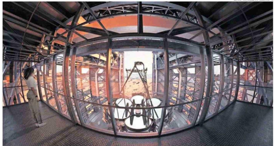
GIGANT MAGELLAN TELESCOPE
